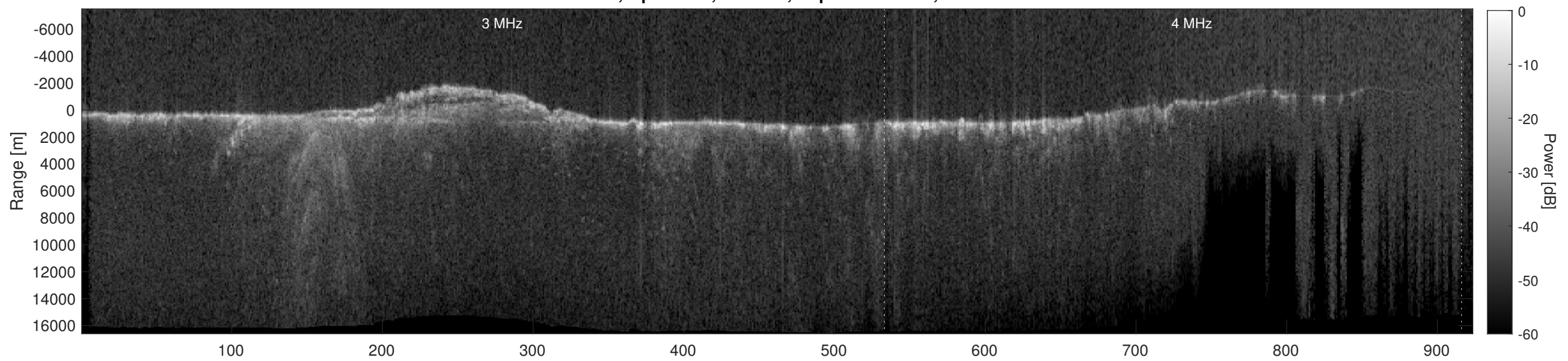
Orbit 11717, Depth-Corrected Cluttergram
