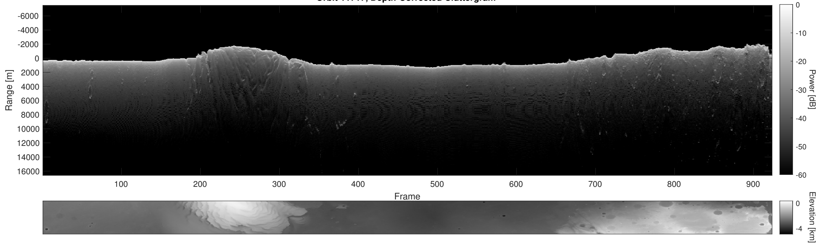
Orbit 11717, Depth-Corrected Cluttergram
