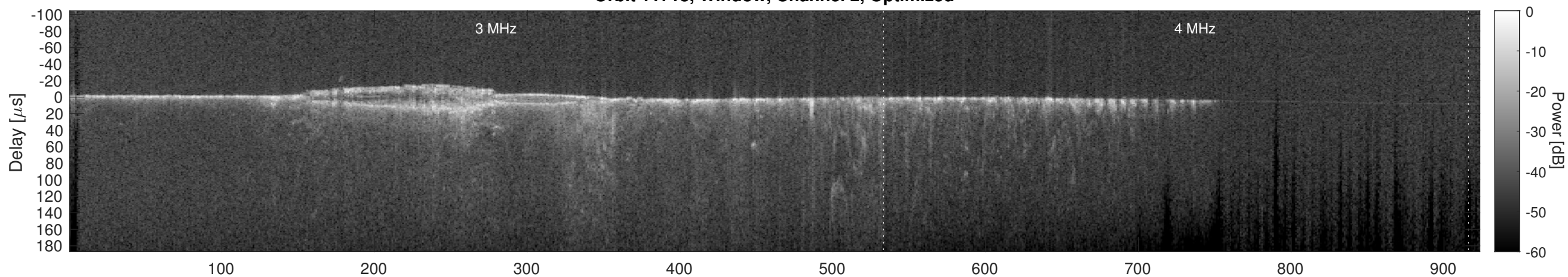
Orbit 11718, Cluttergram
