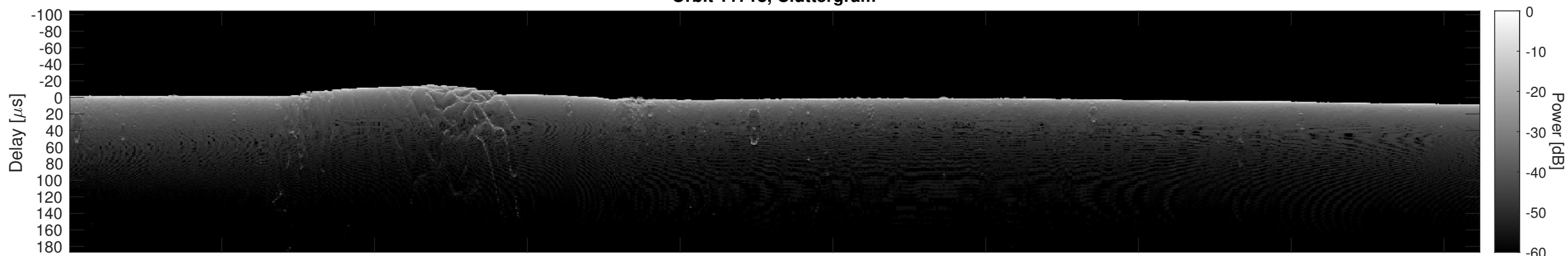
Orbit 11718, Cluttergram
