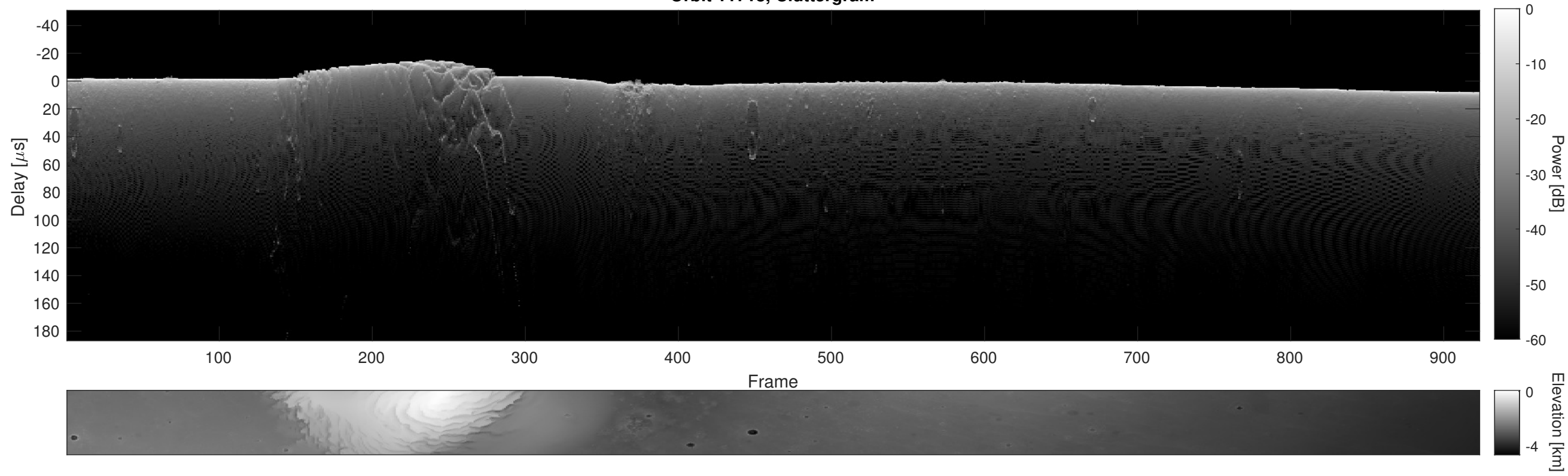
Orbit 11718, Cluttergram
