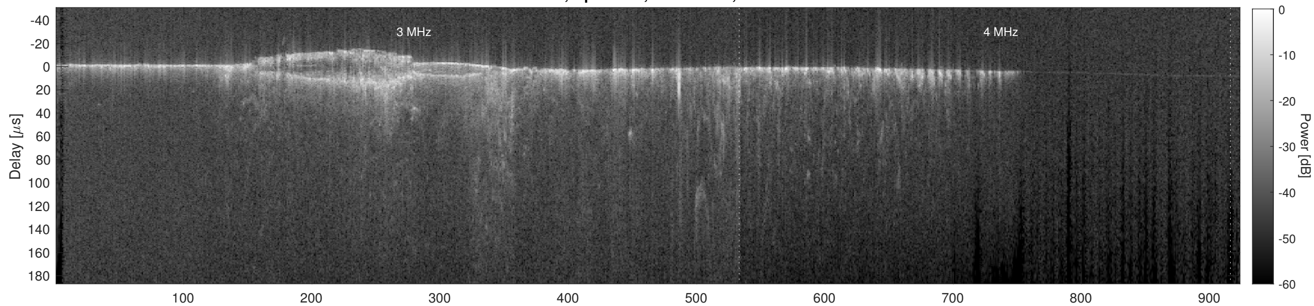
Orbit 11718, Cluttergram
