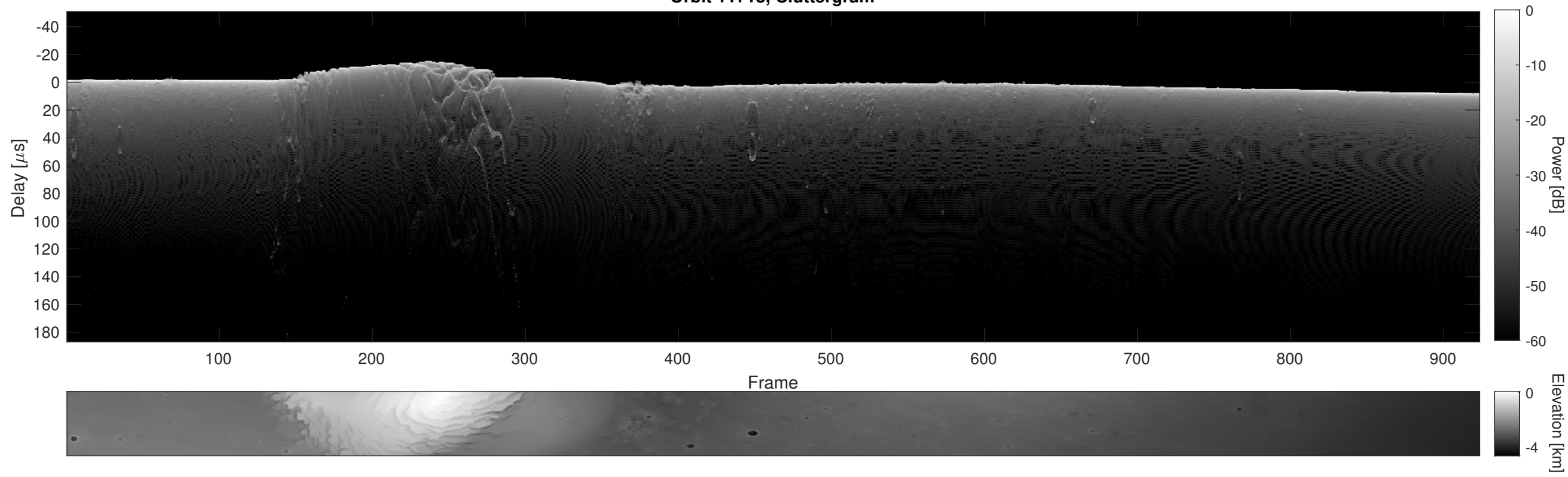
Orbit 11718, Cluttergram
