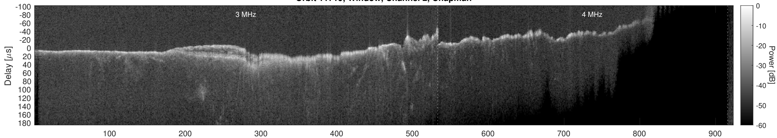
Orbit 11719, Window, Channel 2, Optimized
