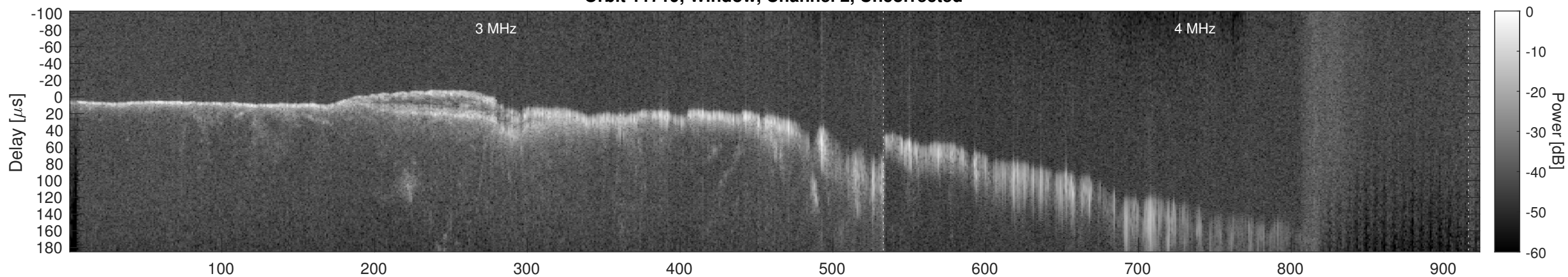
Orbit 11719, Window, Channel 2, Chapman
