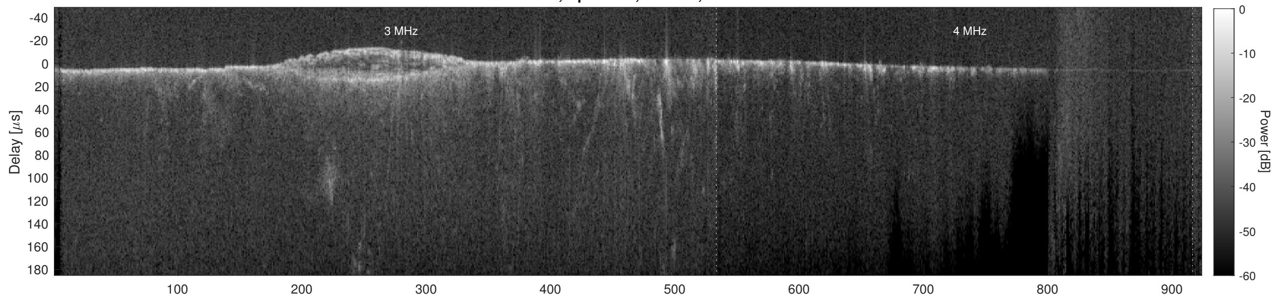
Orbit 11719, Cluttergram
