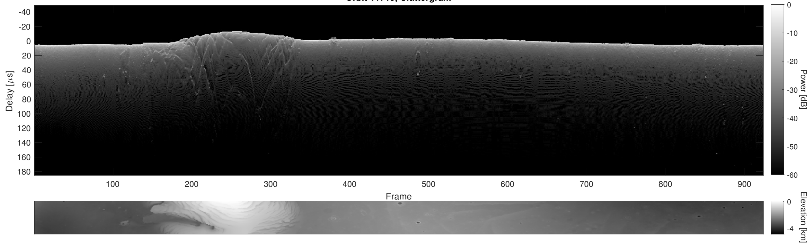
Orbit 11719, Cluttergram
