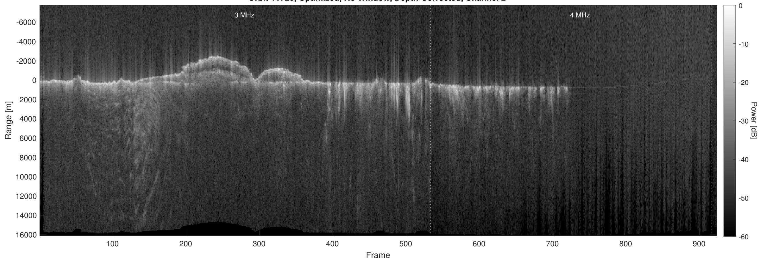
Orbit 11720, Optimized, No Window, Depth-Corrected, Channel 2
