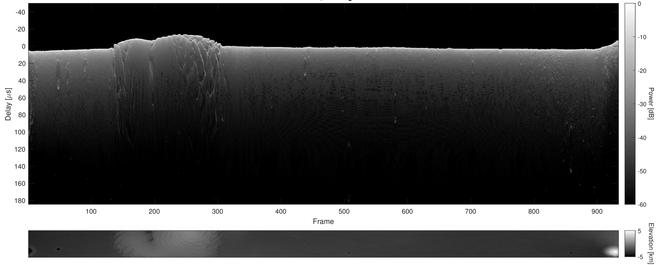
Orbit 11722, Cluttergram
