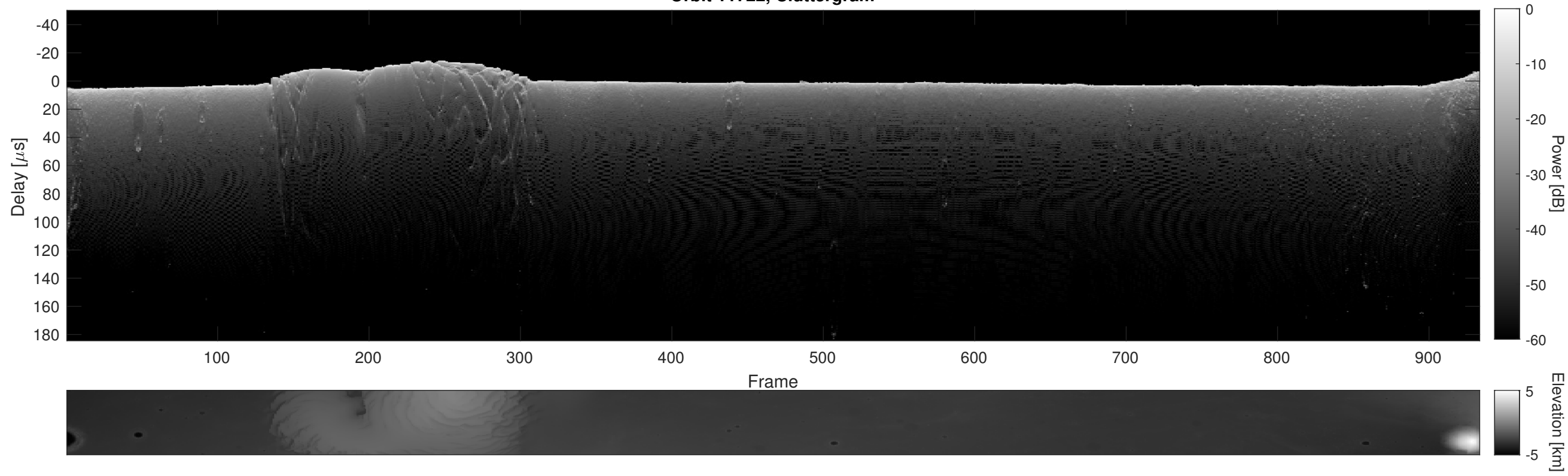
Orbit 11722, Cluttergram
