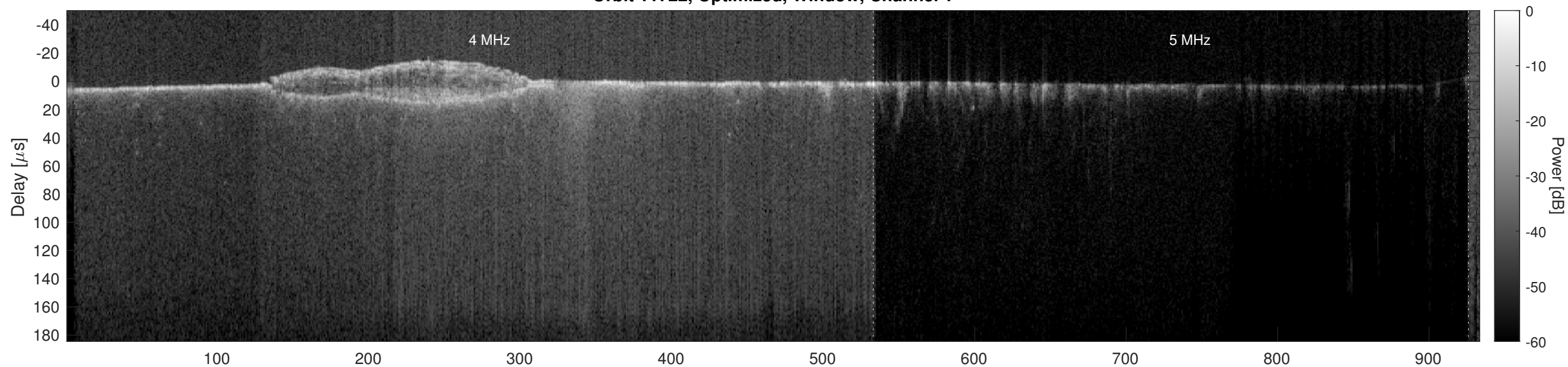
Orbit 11722, Optimized, Window, Channel 2
