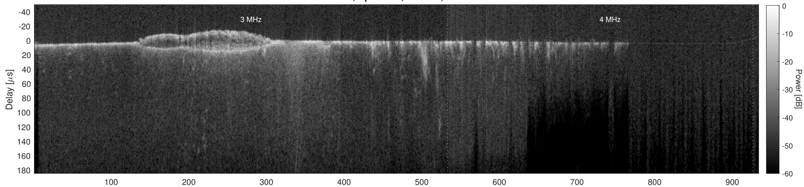
Orbit 11722, Cluttergram
