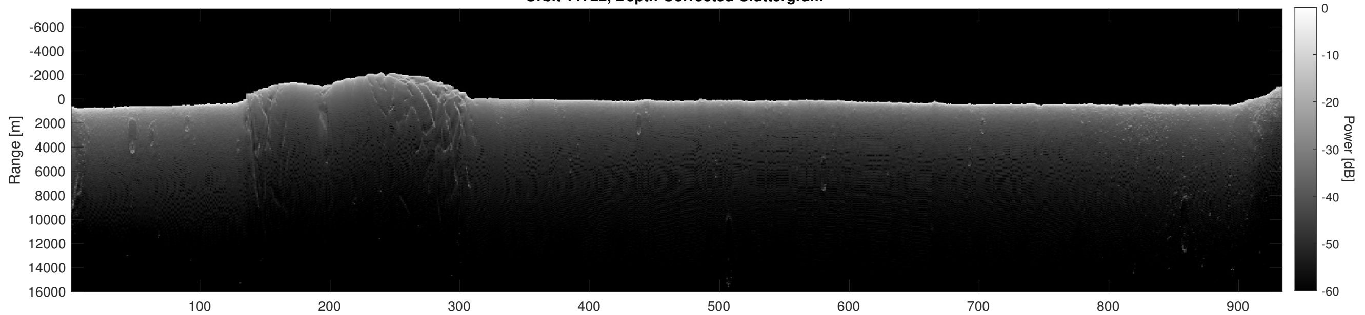
Orbit 11722, Depth-Corrected Cluttergram
