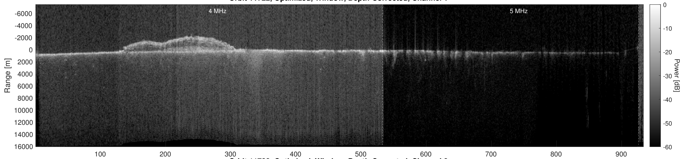
Orbit 11722, Optimized, Window, Depth-Corrected, Channel 2
