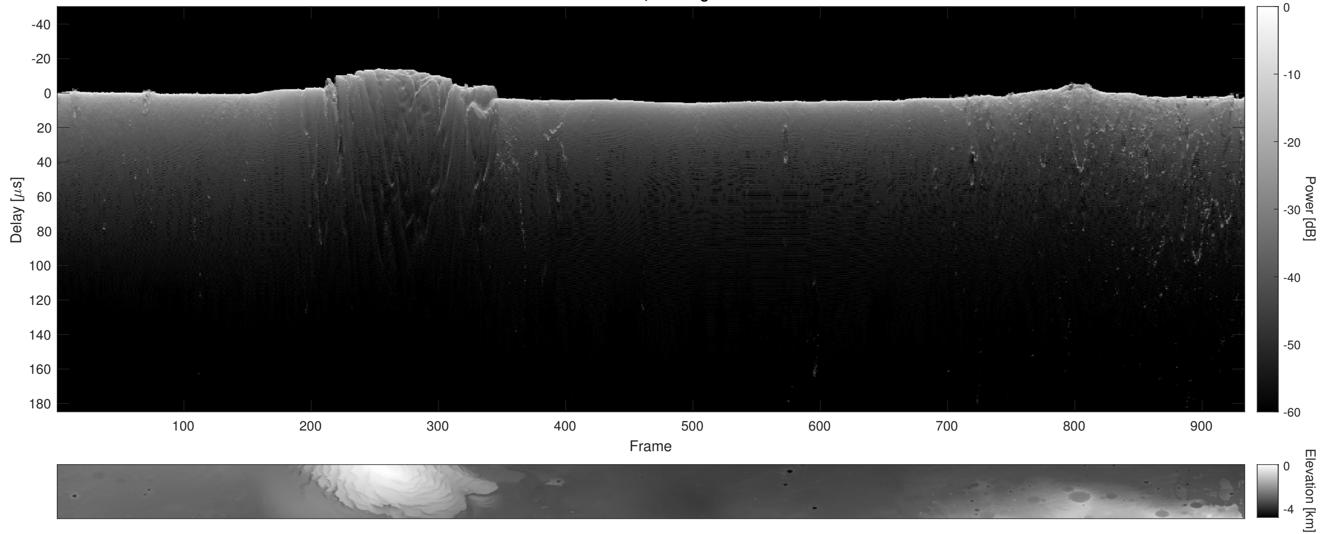
Orbit 11724, Cluttergram
