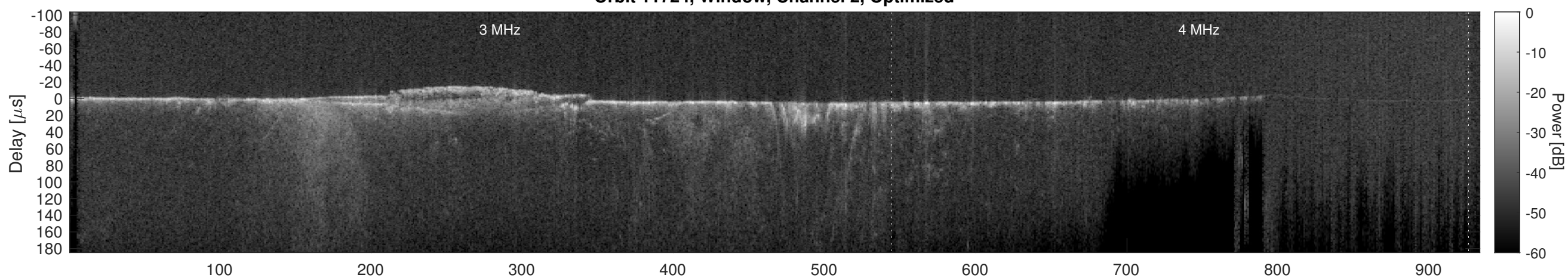
Orbit 11724, Cluttergram
