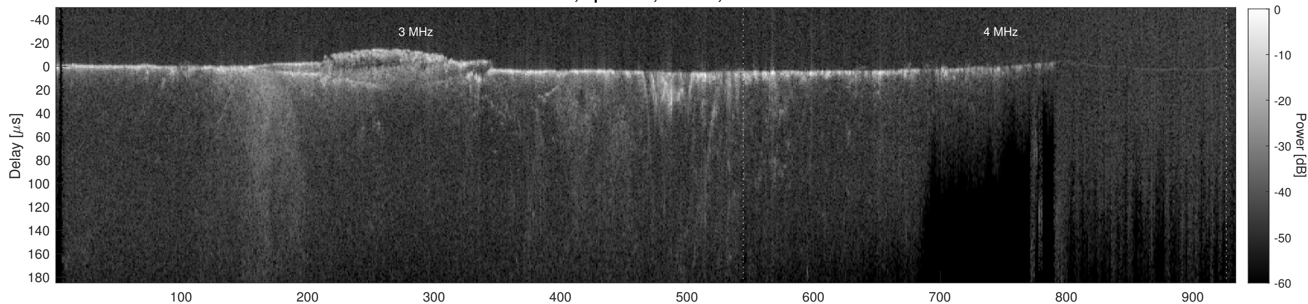
Orbit 11724, Cluttergram
