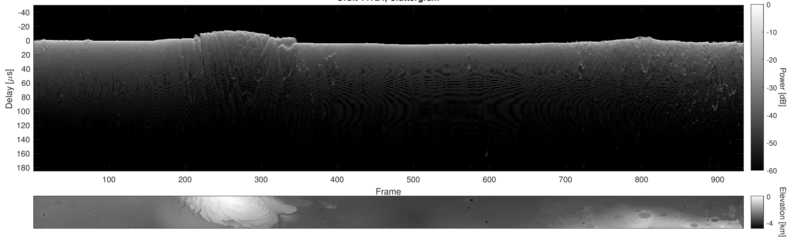
Orbit 11724, Cluttergram
