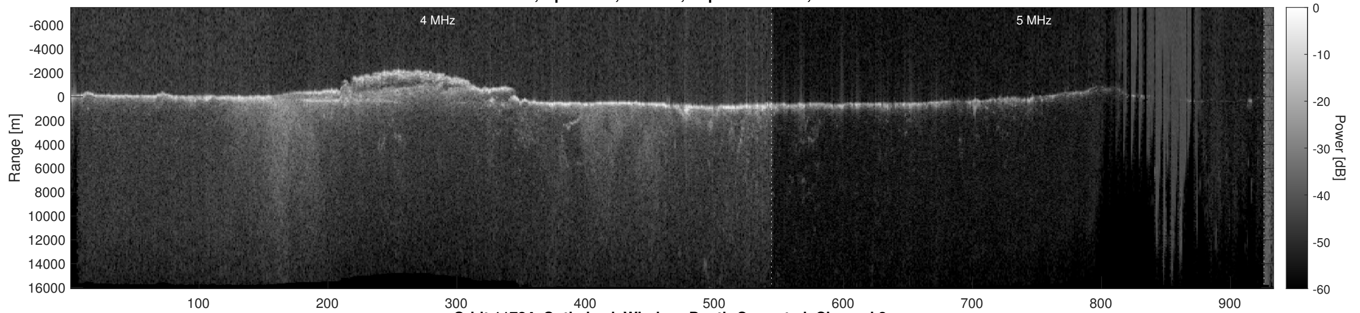
Orbit 11724, Optimized, Window, Depth-Corrected, Channel 2
