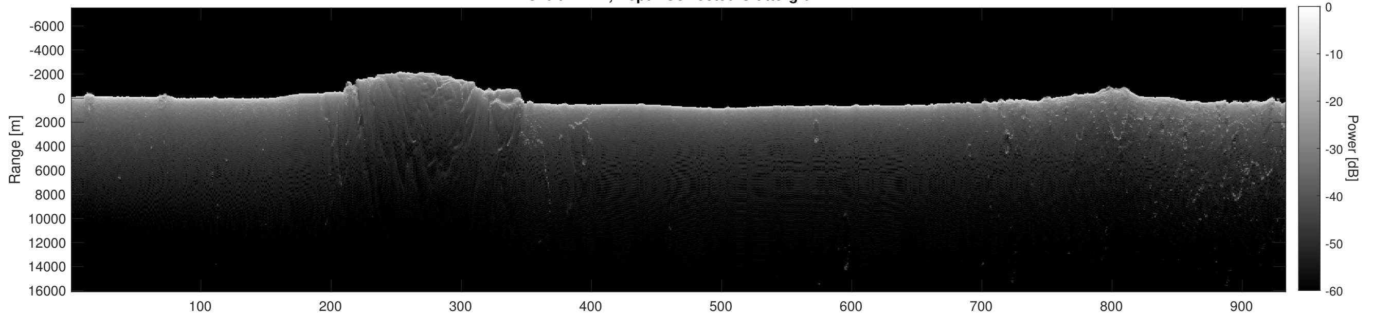
Orbit 11724, Depth-Corrected Cluttergram
