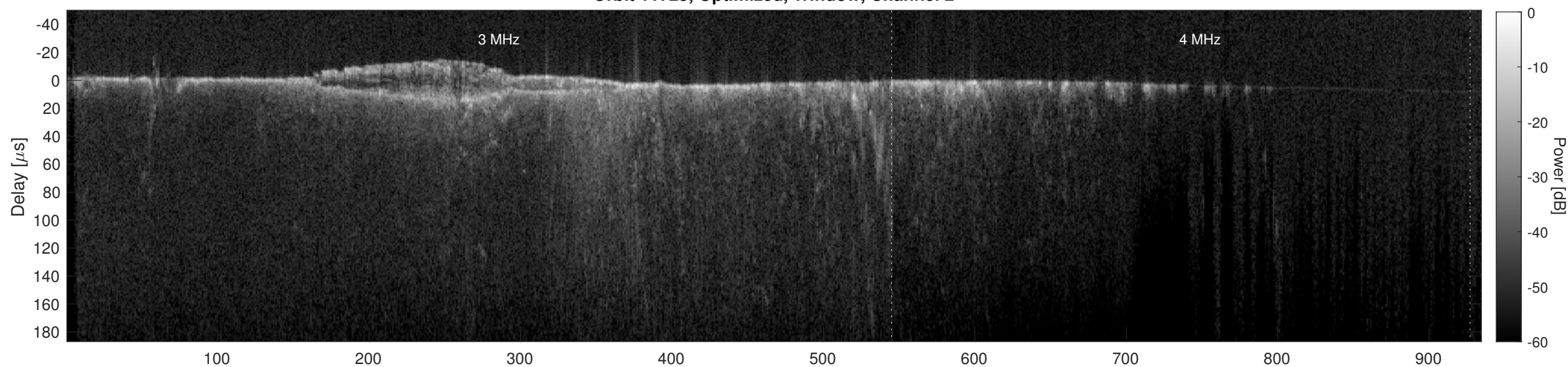
Orbit 11725, Cluttergram
