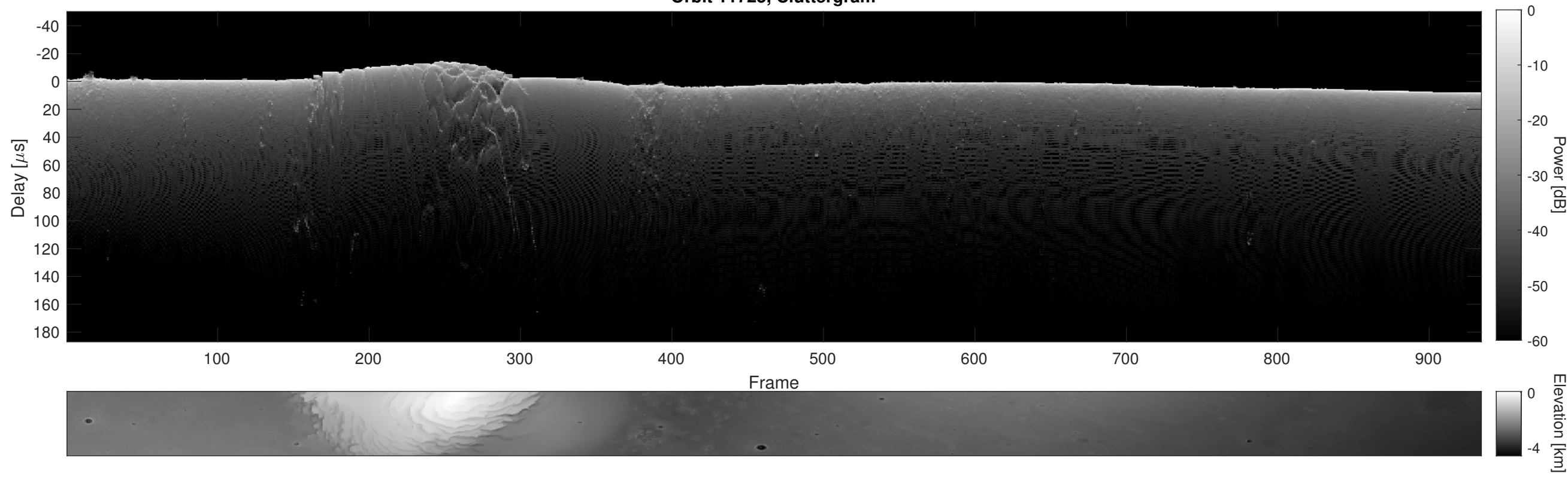
Orbit 11725, Cluttergram
