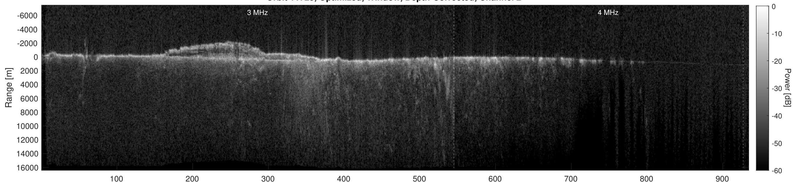
Orbit 11725, Depth-Corrected Cluttergram
