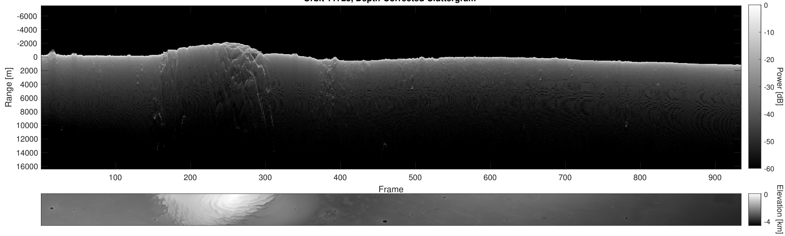
Orbit 11725, Depth-Corrected Cluttergram
