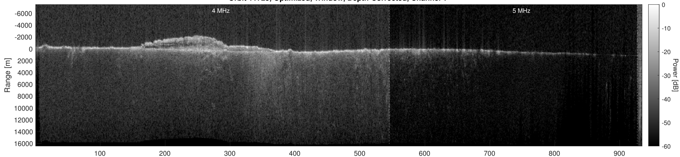
Orbit 11725, Optimized, Window, Depth-Corrected, Channel 2
