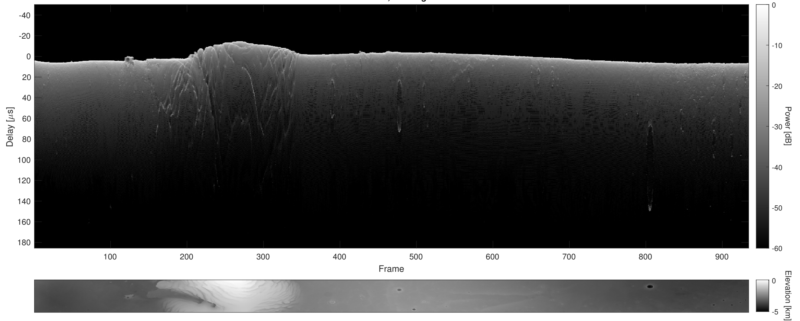
Orbit 11726, Cluttergram
