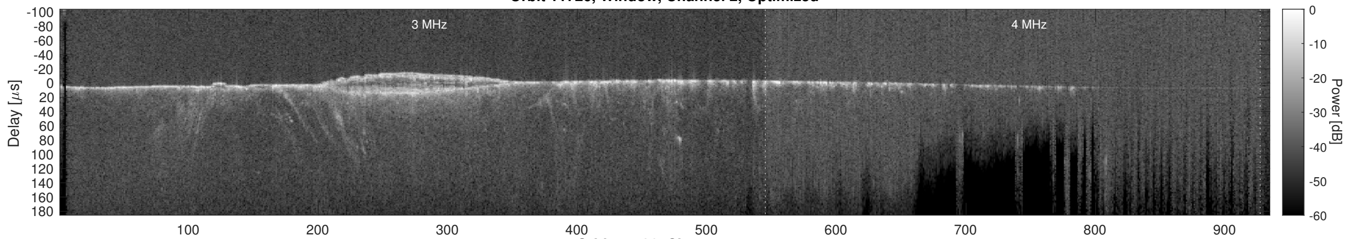
Orbit 11726, Cluttergram
