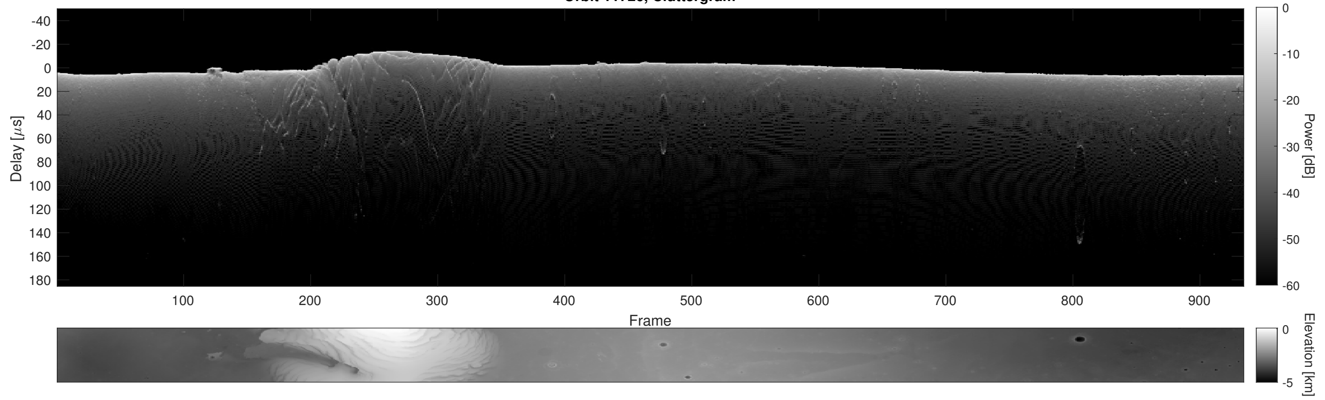
Orbit 11726, Cluttergram
