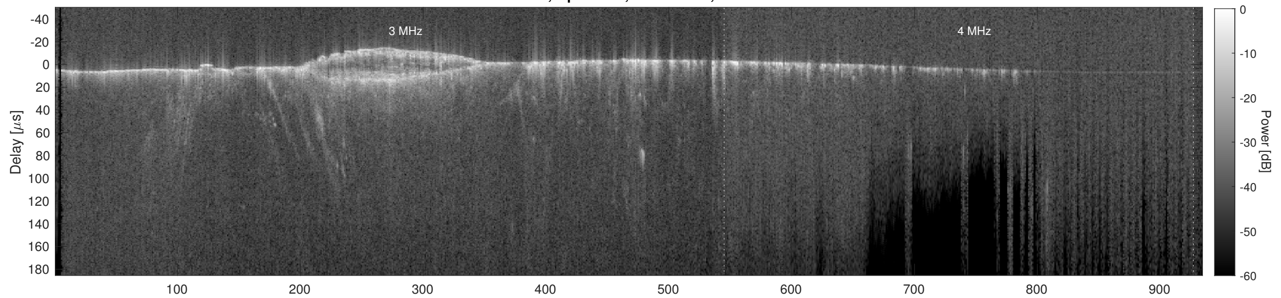
Orbit 11726, Cluttergram
