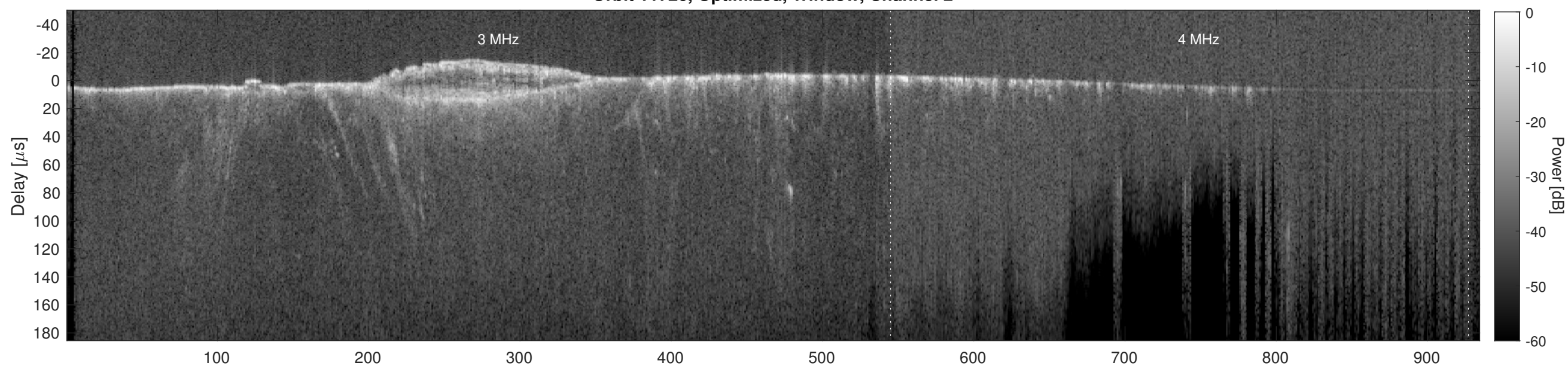
Orbit 11726, Cluttergram
