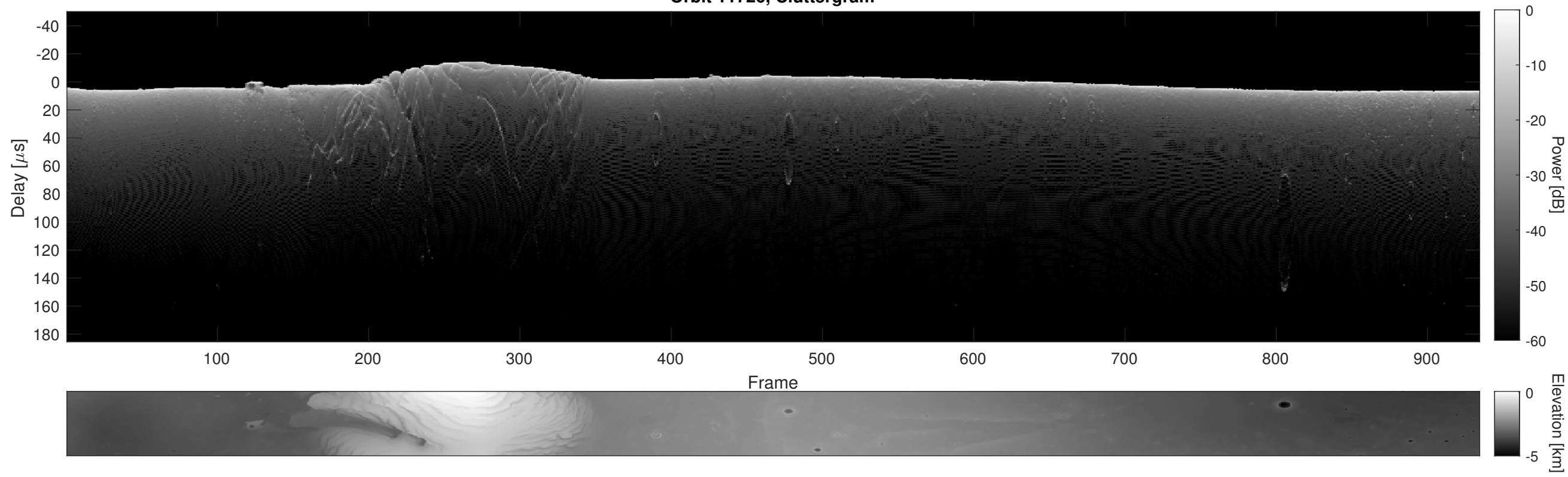
Orbit 11726, Cluttergram
