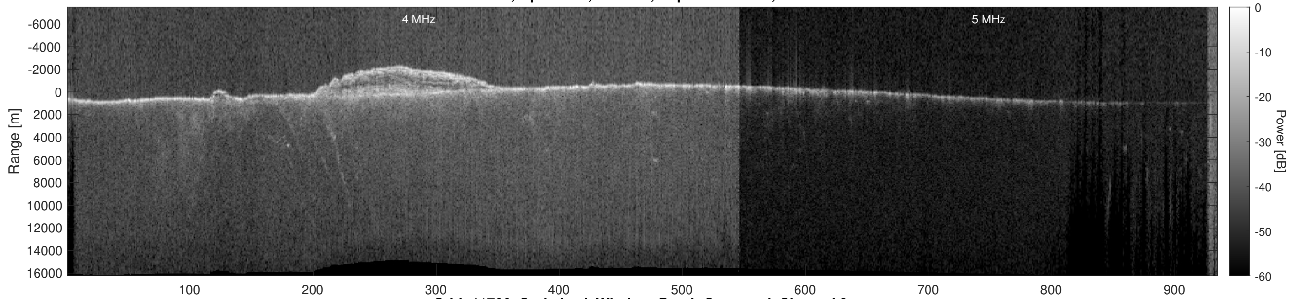
Orbit 11726, Optimized, Window, Depth-Corrected, Channel 2
