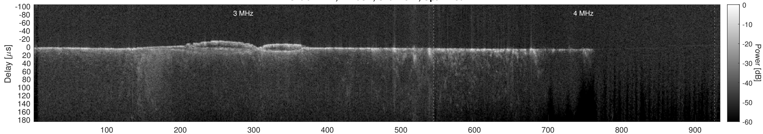
Orbit 11727, Cluttergram
