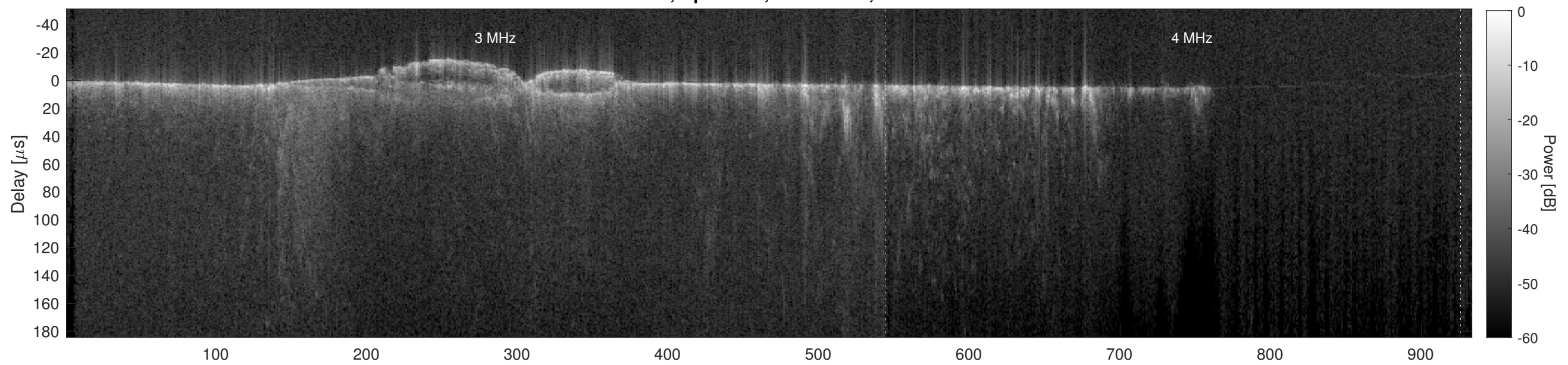
Orbit 11727, Cluttergram
