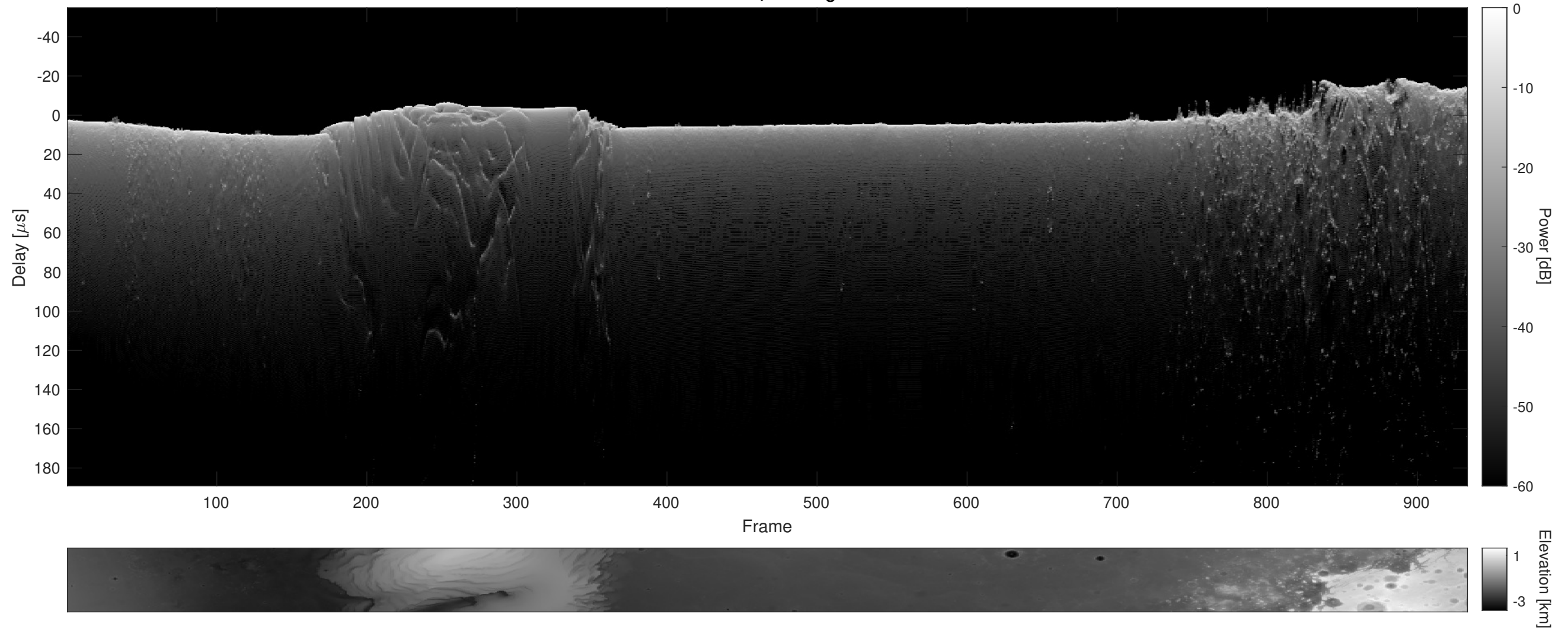
Orbit 11730, Cluttergram
