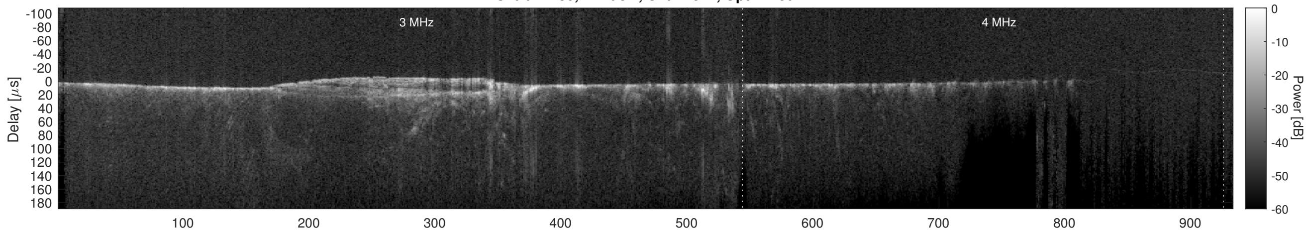
Orbit 11730, Cluttergram
