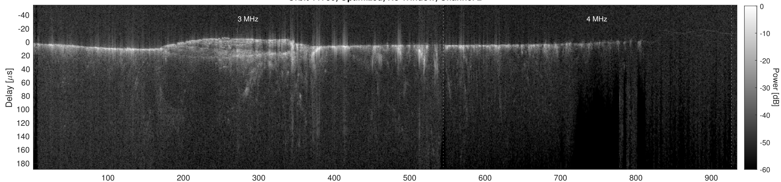
Orbit 11730, Cluttergram
