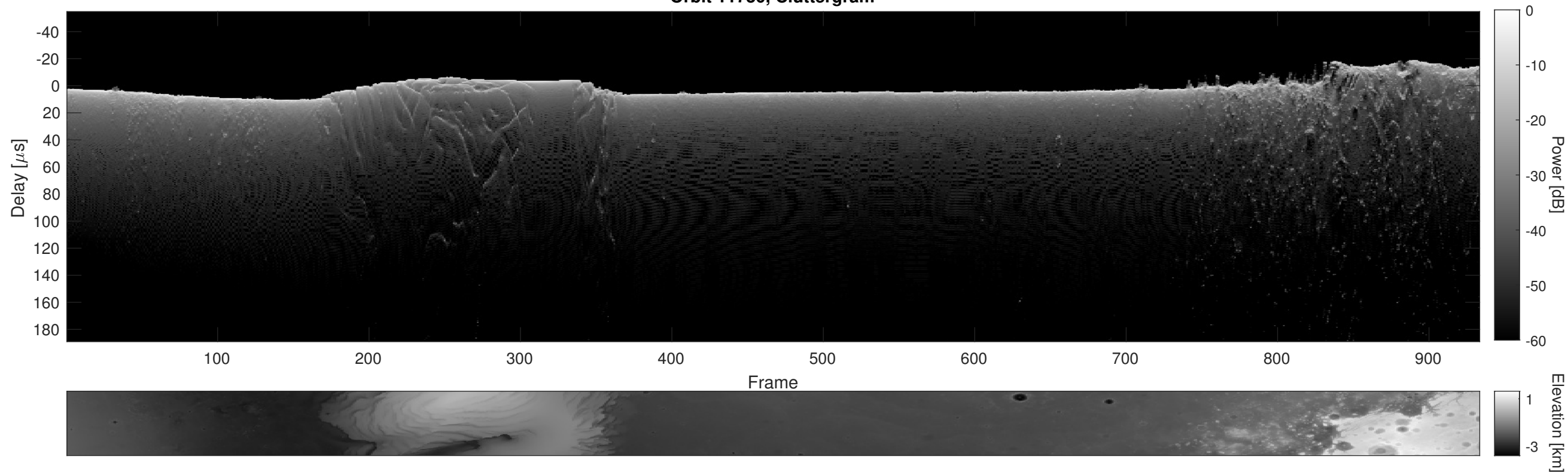
Orbit 11730, Cluttergram
