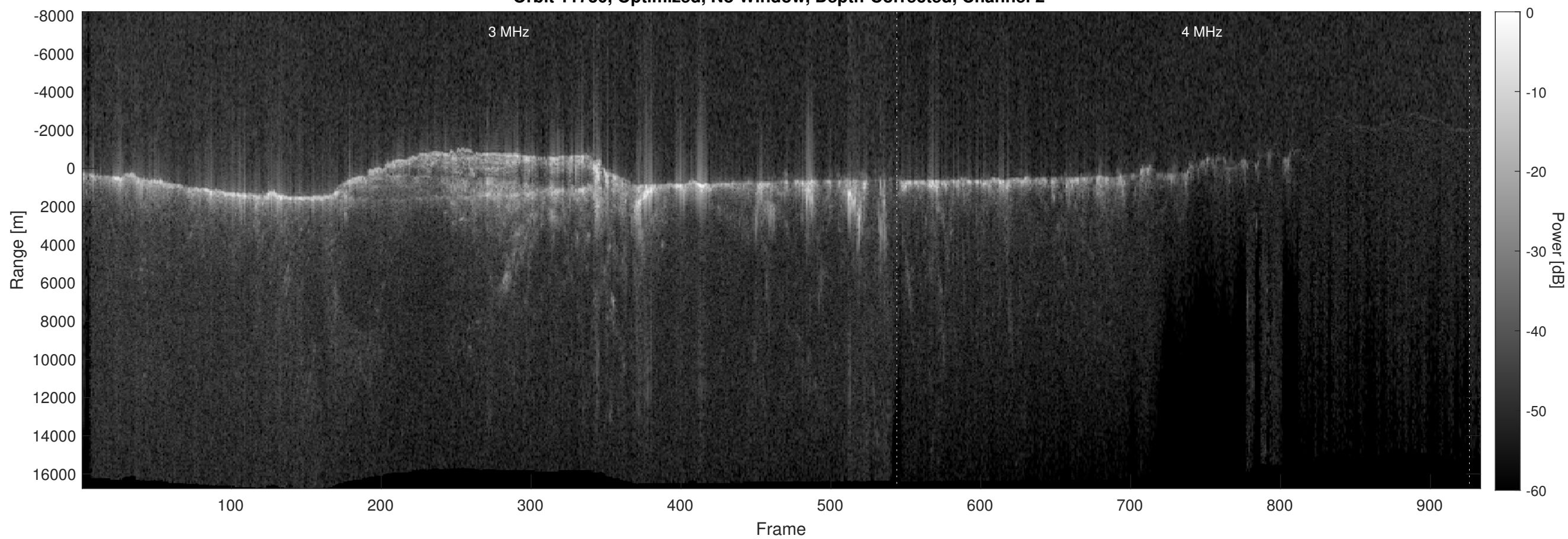
Orbit 11730, Optimized, No Window, Depth-Corrected, Channel 2
