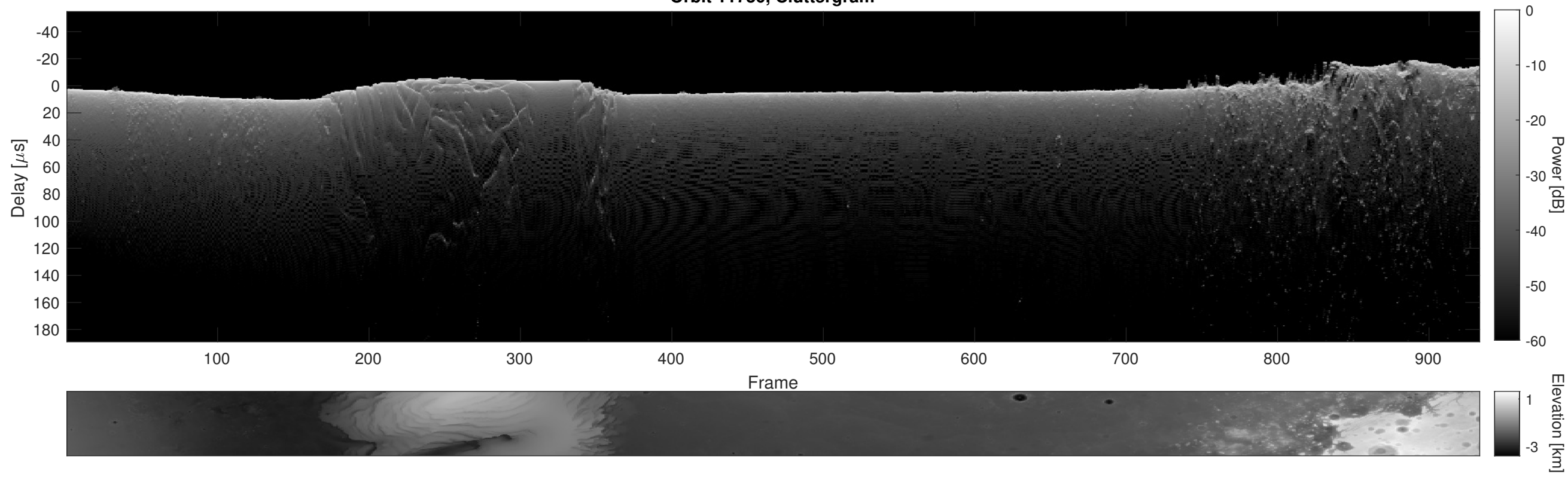
Orbit 11730, Cluttergram
