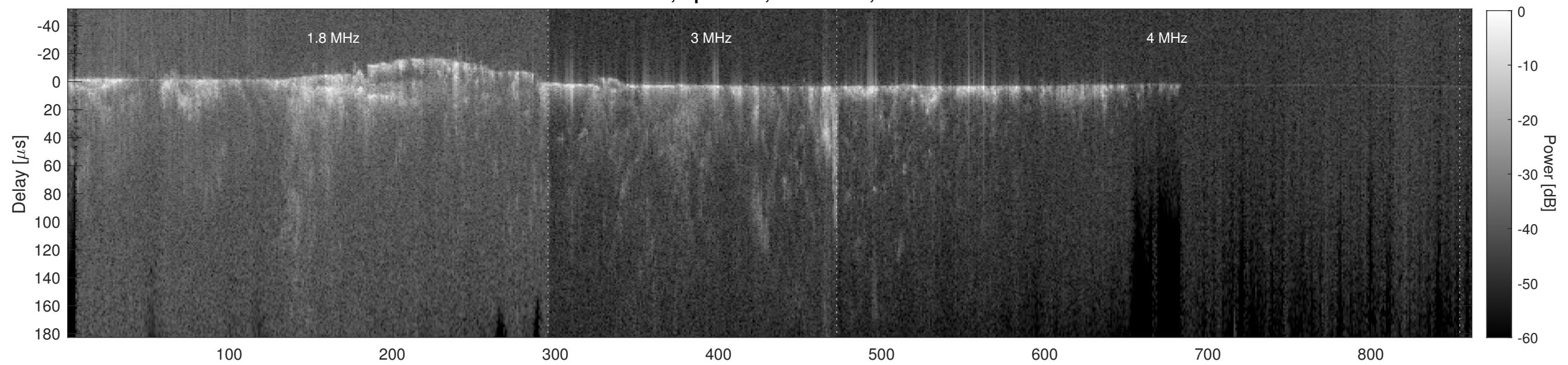
Orbit 11731, Cluttergram
