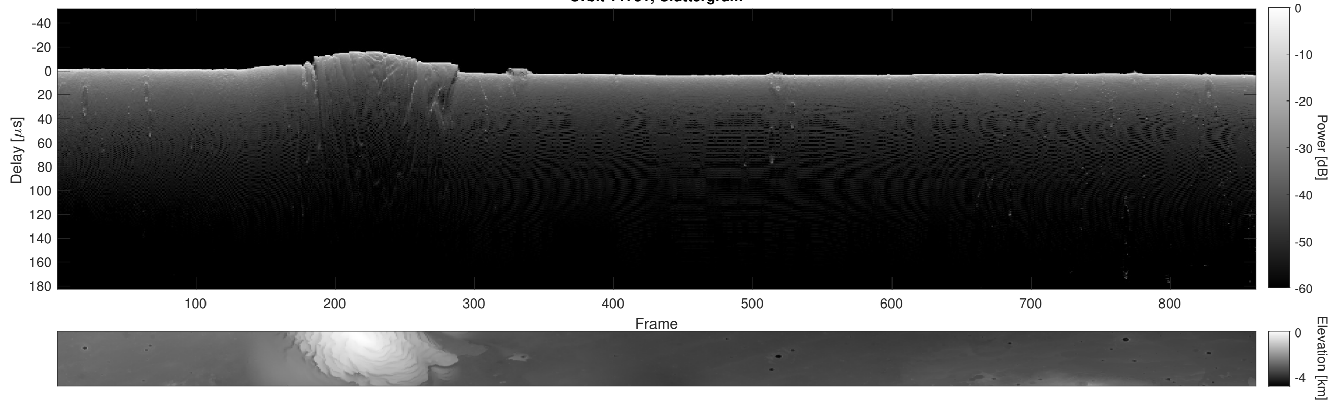
Orbit 11731, Cluttergram
