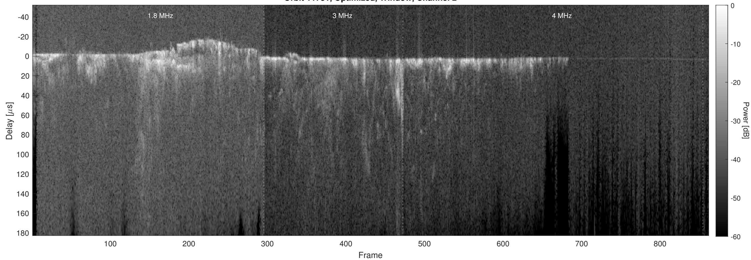
Orbit 11731, Optimized, Window, Channel 2
