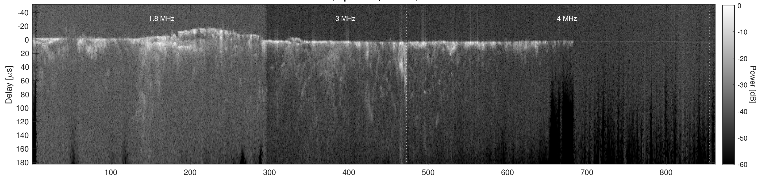
Orbit 11731, Cluttergram
