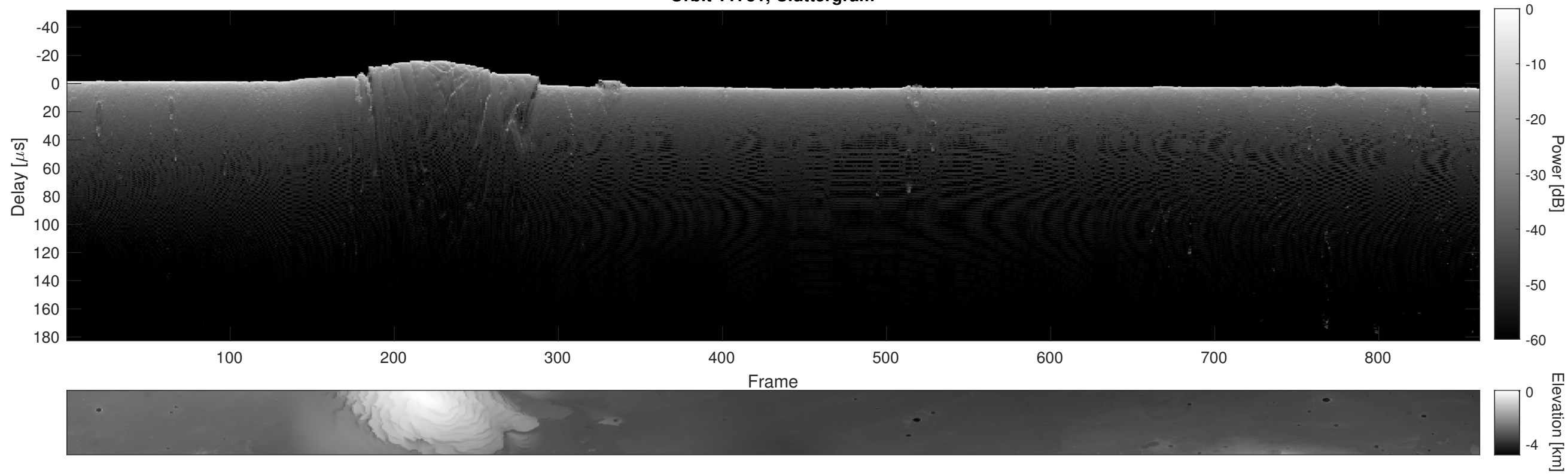
Orbit 11731, Cluttergram
