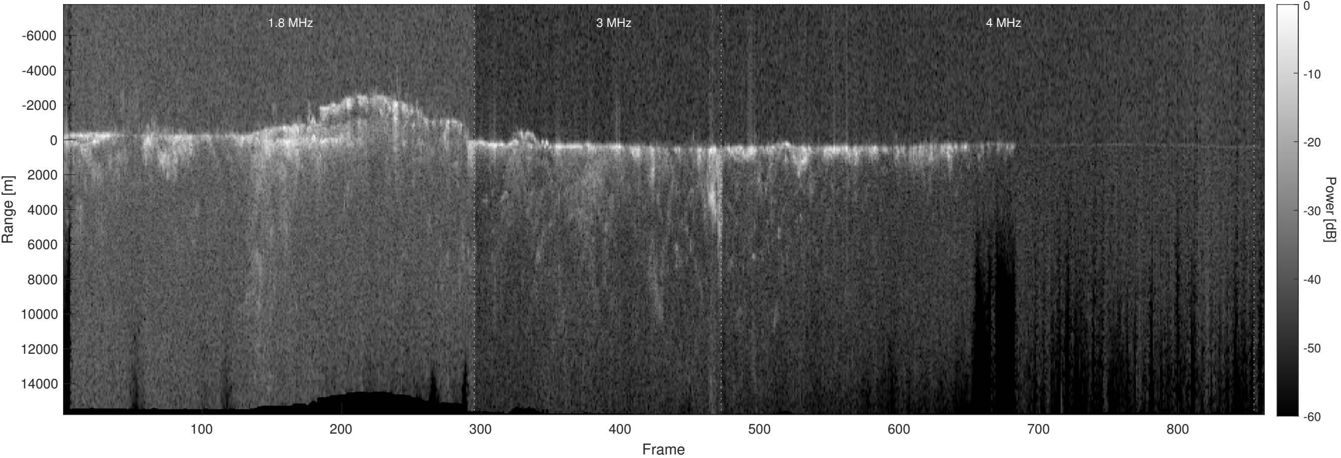
Orbit 11731, Optimized, Window, Depth-Corrected, Channel 2
