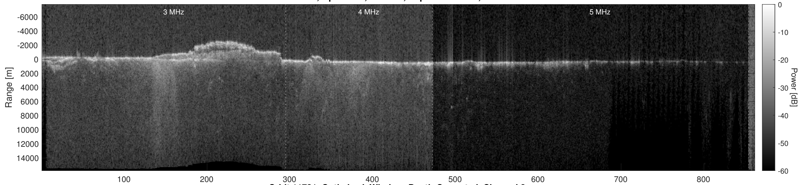
Orbit 11731, Optimized, Window, Depth-Corrected, Channel 2
