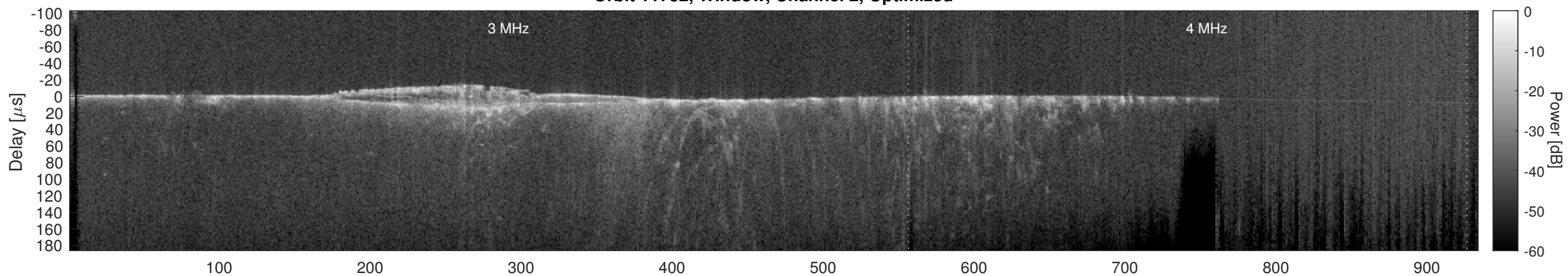
Orbit 11732, Cluttergram
