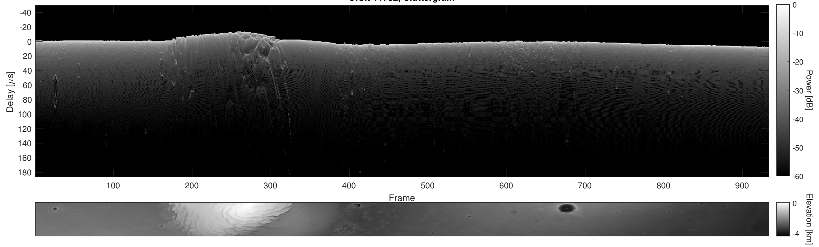
Orbit 11732, Cluttergram
