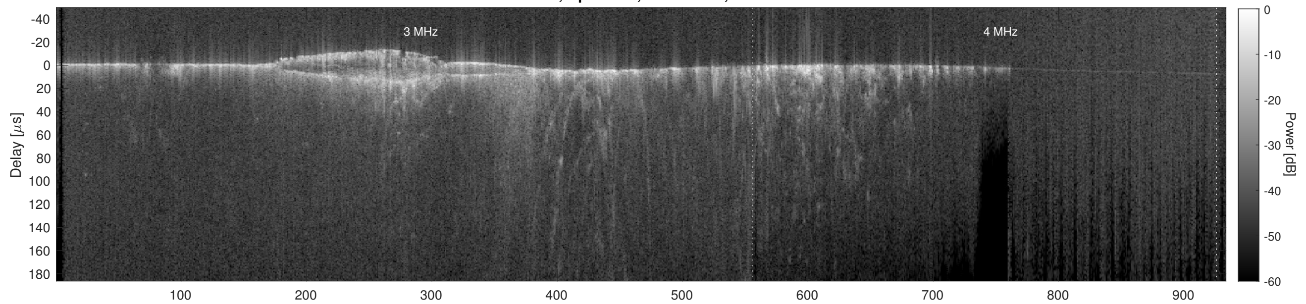
Orbit 11732, Cluttergram
