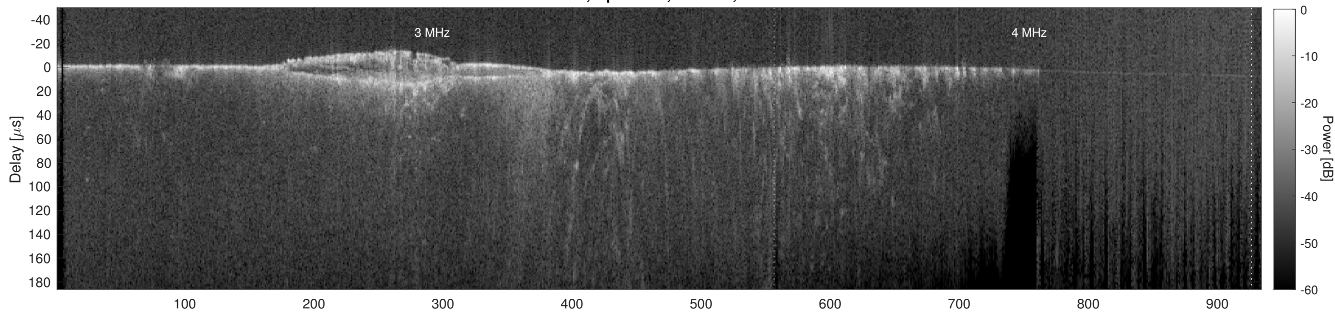
Orbit 11732, Cluttergram
