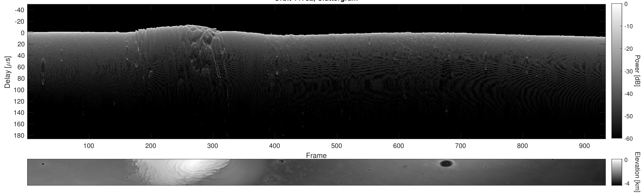
Orbit 11732, Cluttergram
