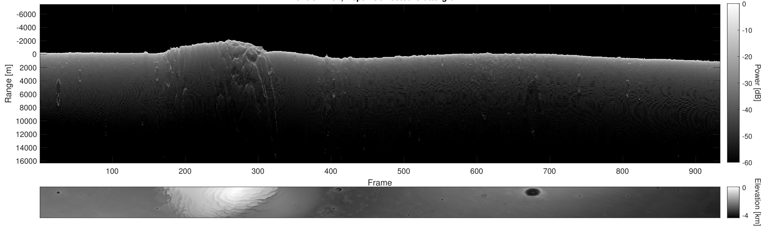
Orbit 11732, Depth-Corrected Cluttergram
