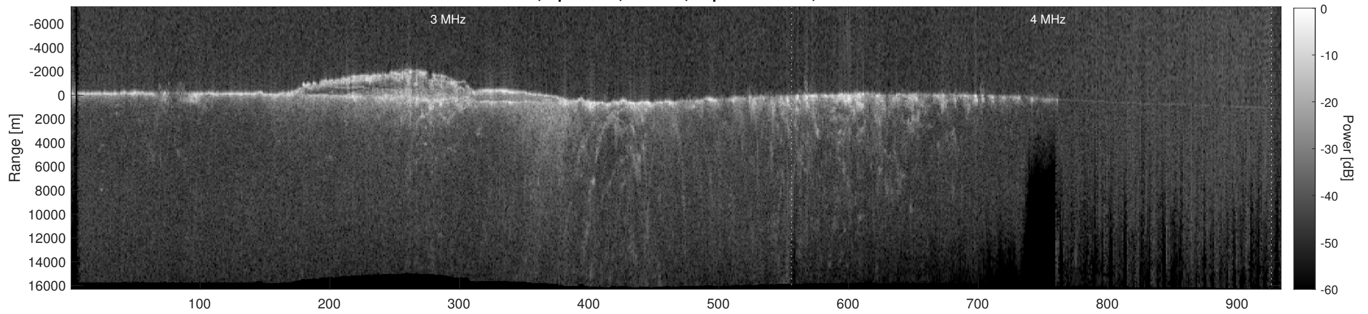
Orbit 11732, Depth-Corrected Cluttergram
