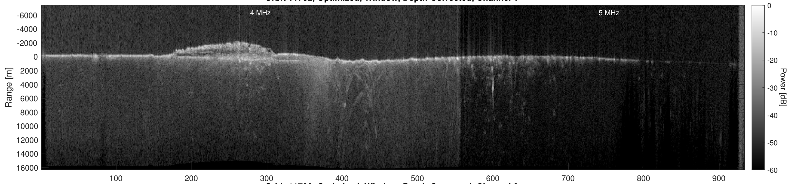
Orbit 11732, Optimized, Window, Depth-Corrected, Channel 2
