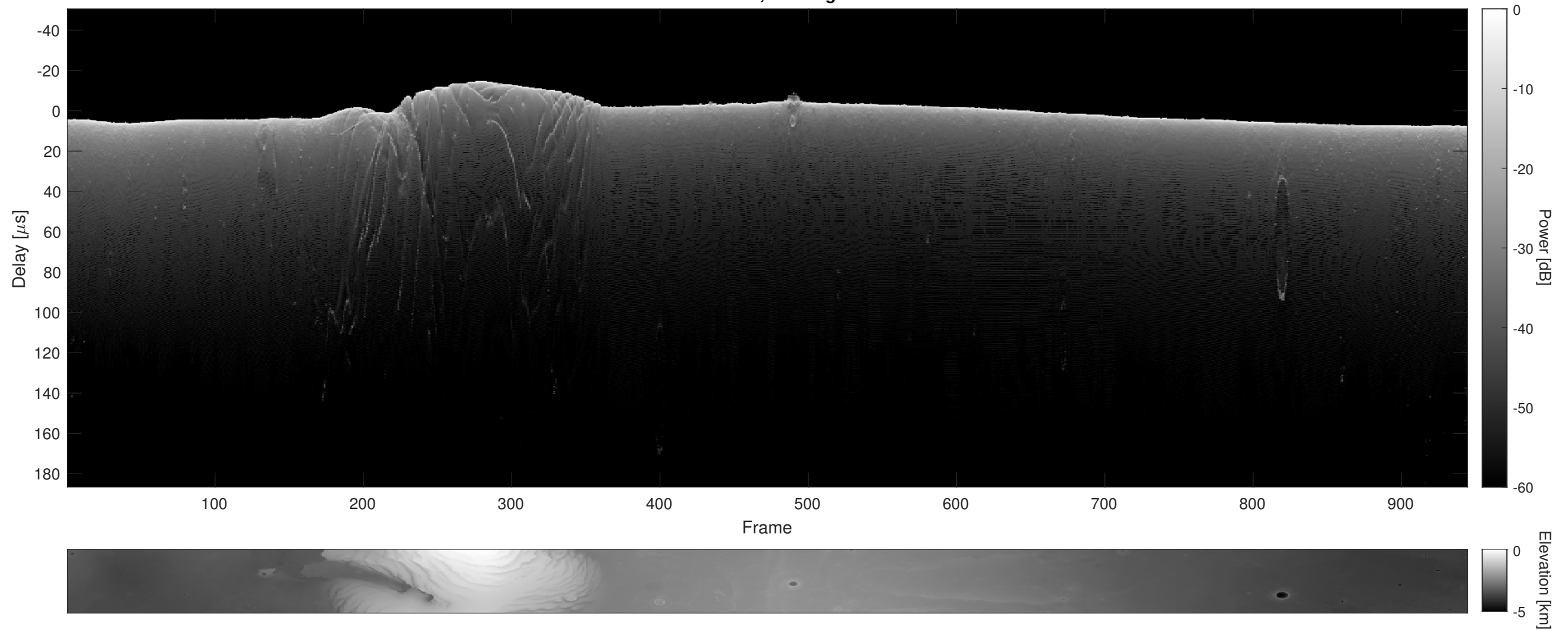
Orbit 11733, Cluttergram
