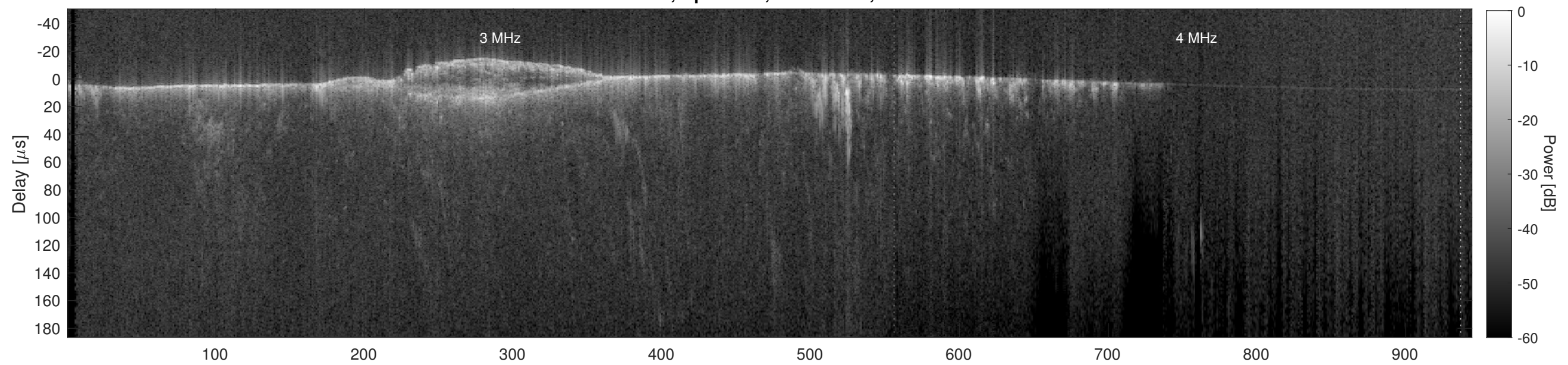
Orbit 11733, Cluttergram
