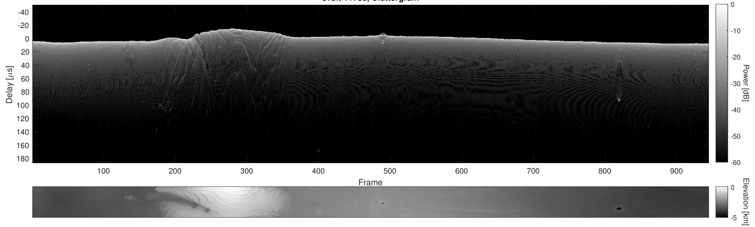
Orbit 11733, Cluttergram
