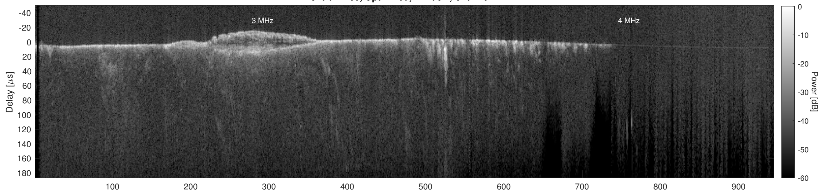
Orbit 11733, Cluttergram
