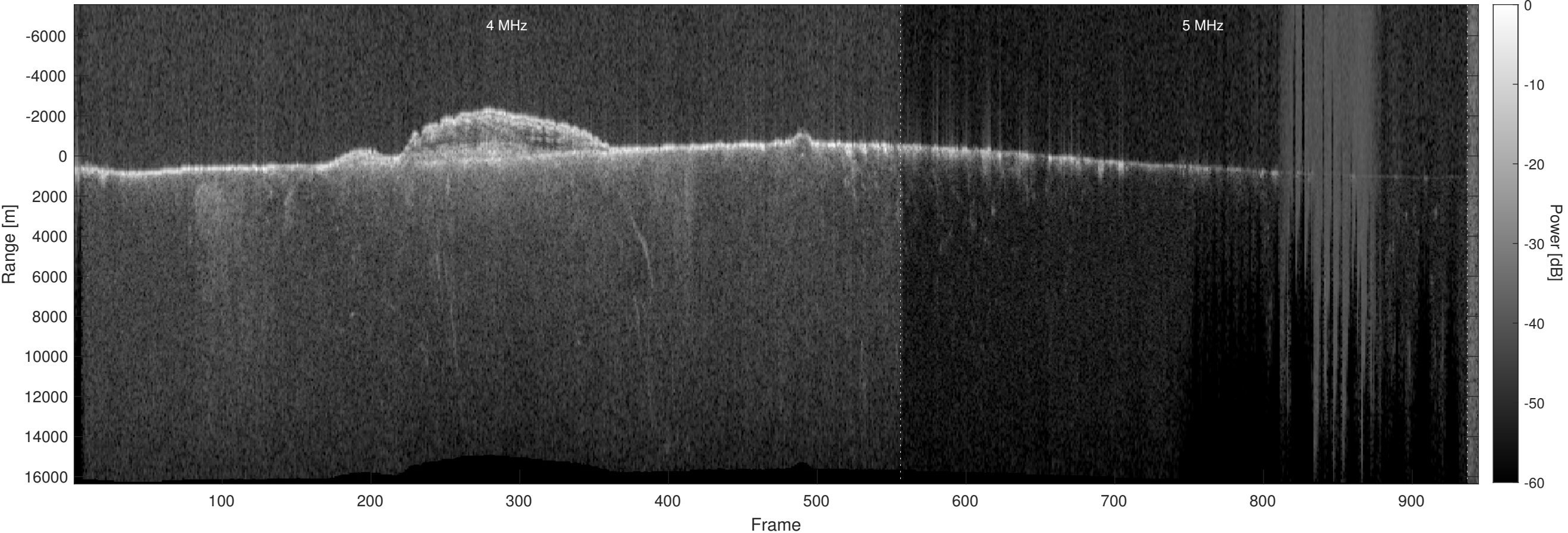
Orbit 11733, Optimized, Window, Depth-Corrected, Channel 2
