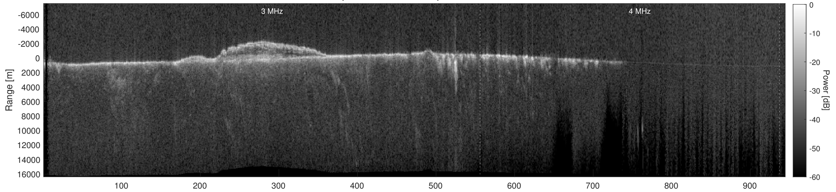
Orbit 11733, Depth-Corrected Cluttergram
