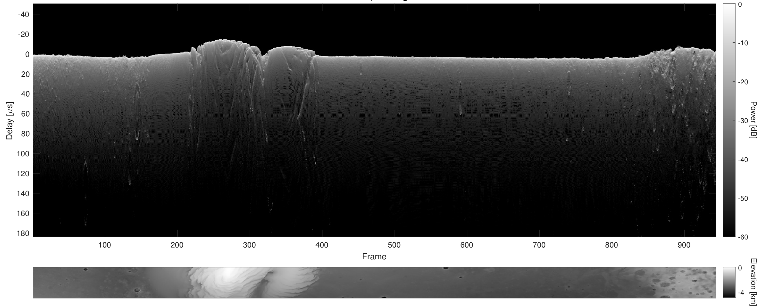
Orbit 11734, Cluttergram
