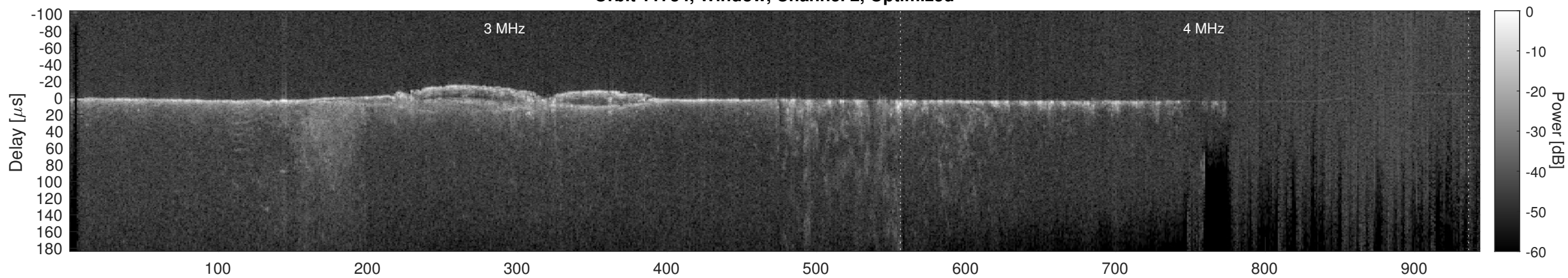
Orbit 11734, Cluttergram
