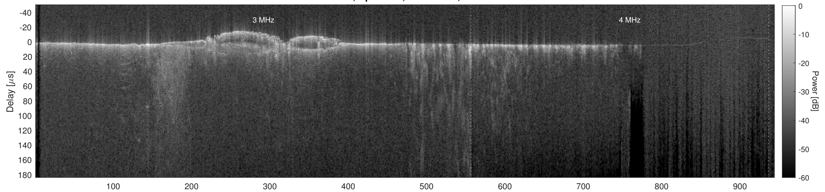
Orbit 11734, Cluttergram
