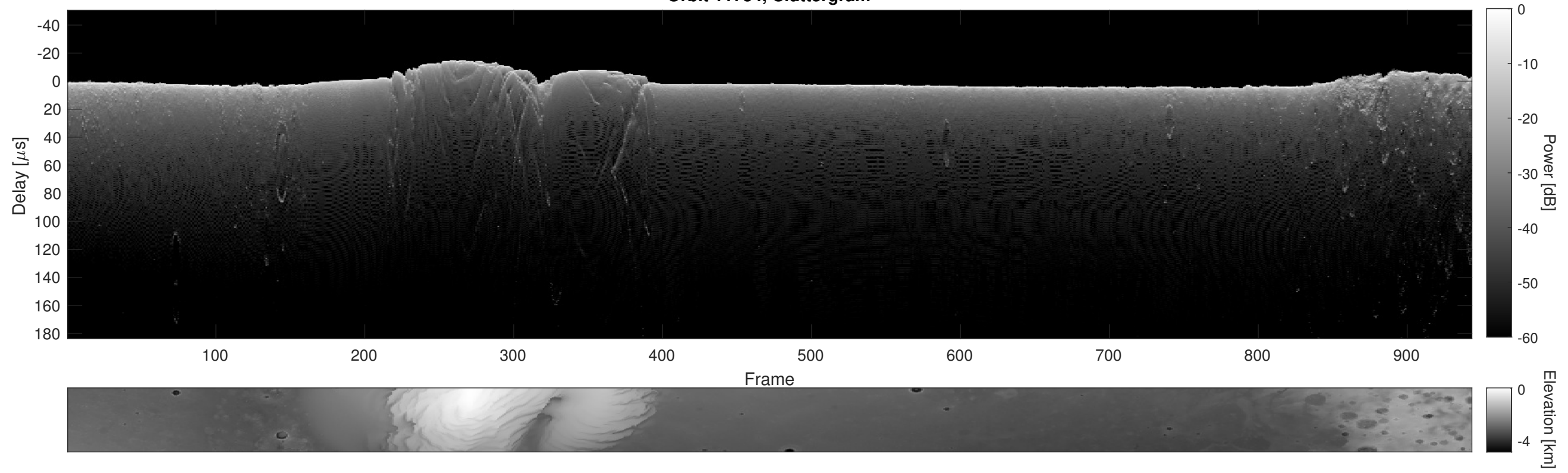
Orbit 11734, Cluttergram
