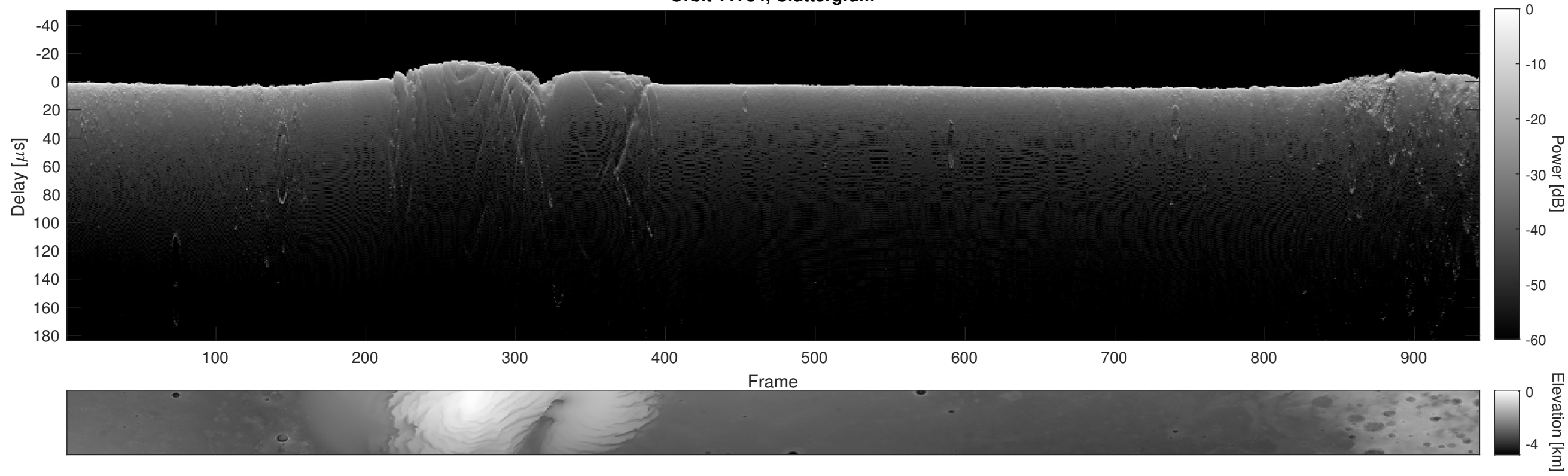
Orbit 11734, Cluttergram
