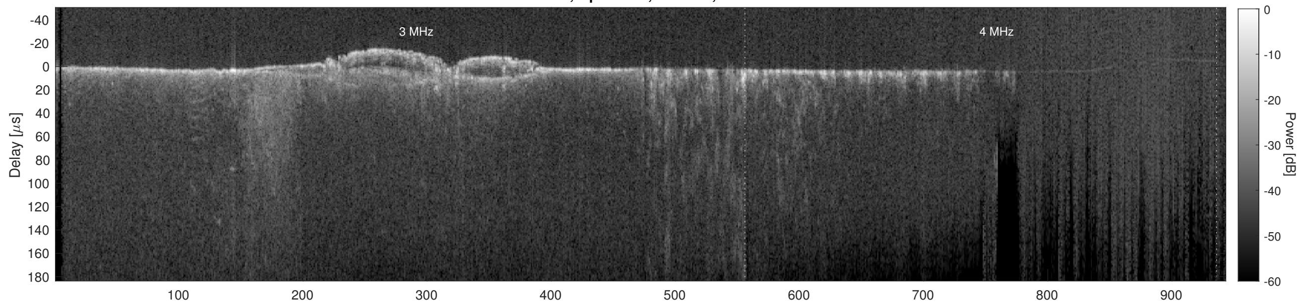
Orbit 11734, Cluttergram
