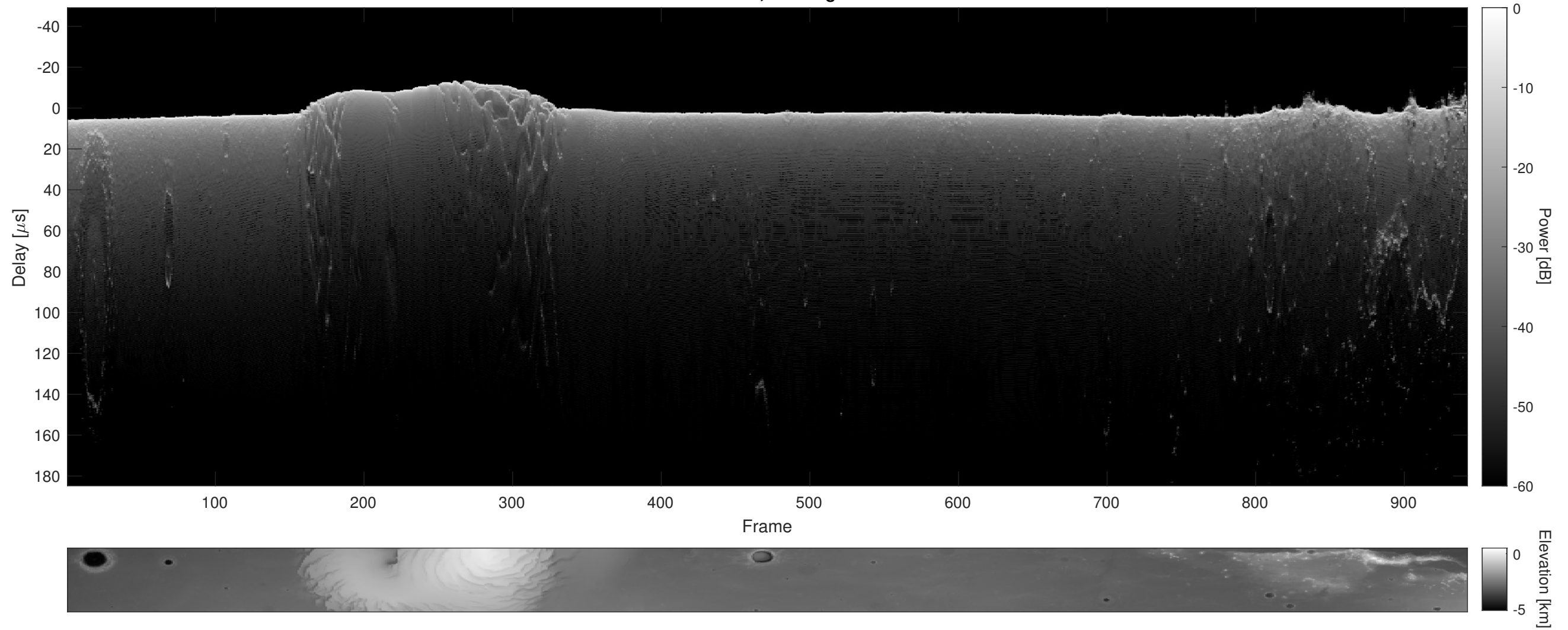
Orbit 11736, Cluttergram
