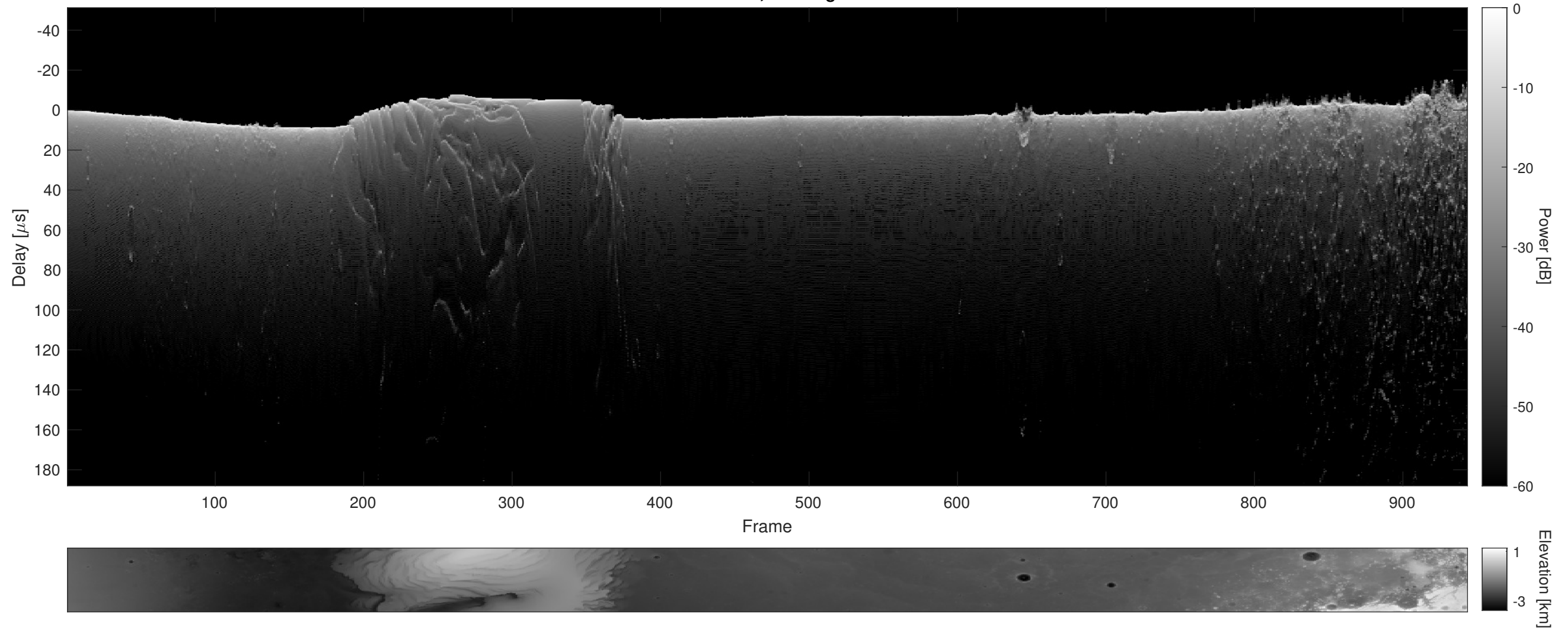
Orbit 11737, Cluttergram
