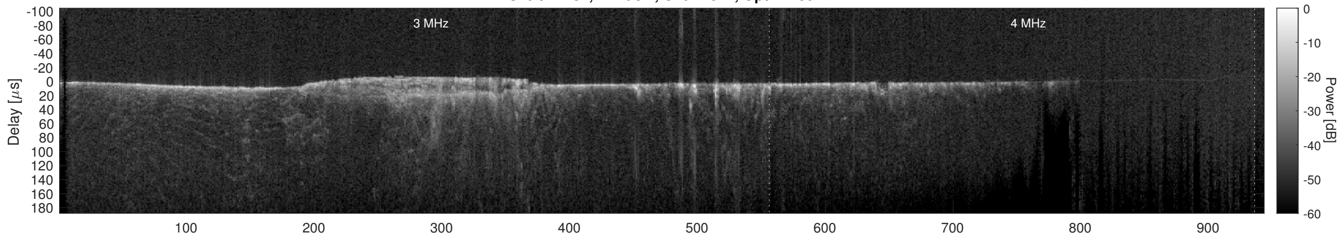
Orbit 11737, Cluttergram
