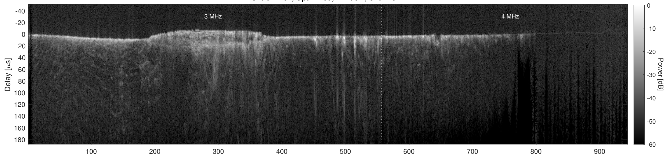
Orbit 11737, Cluttergram
