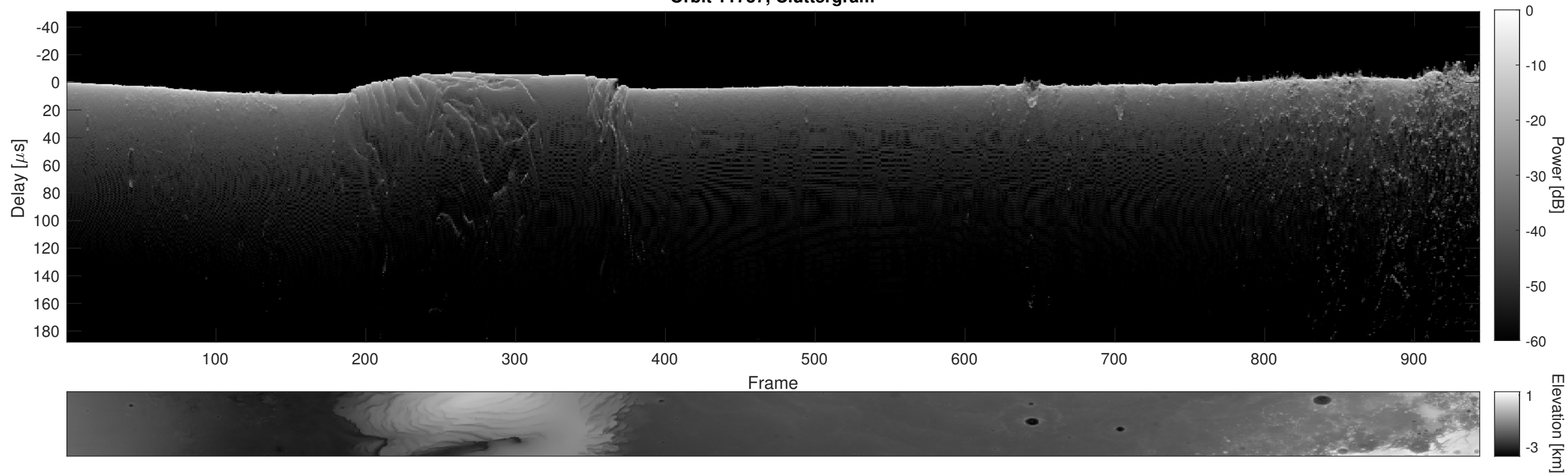
Orbit 11737, Cluttergram
